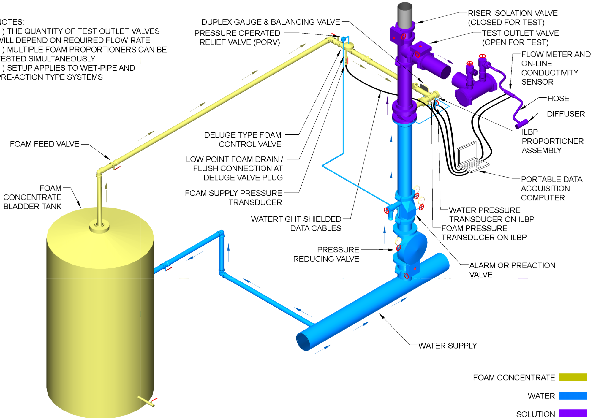
Drawing - VFTDW105 2018-12-14
